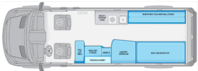
Wave for 2 Daytime Configuration
