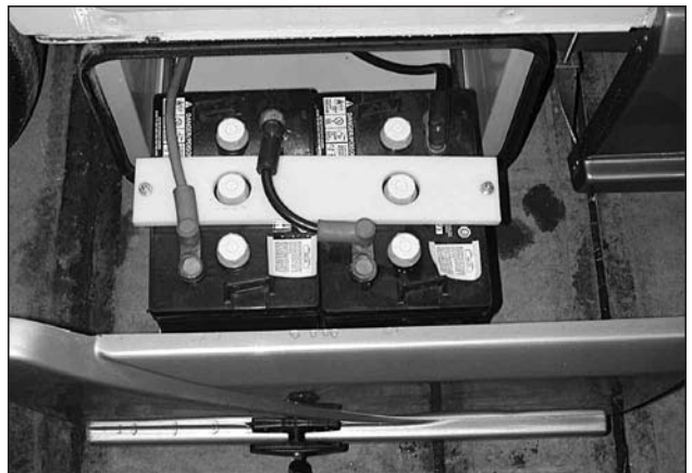
Picture B-P43: Dual battery arrangement and connections.
