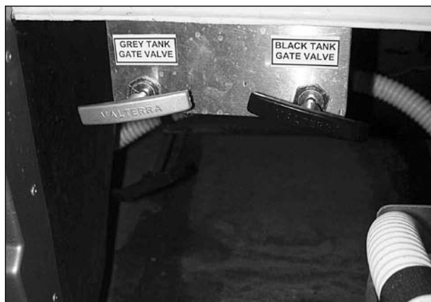
Picture G-P14: Access to sewer discharge assembly, black and grey gate valve handles.
