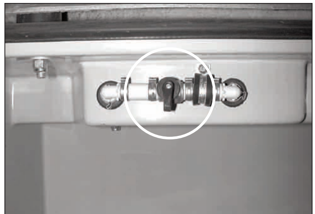
Picture G-P12: Closed position of the city water tank fill valve.
