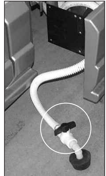
Picture G-P18: Sewage hose discharge valve.
