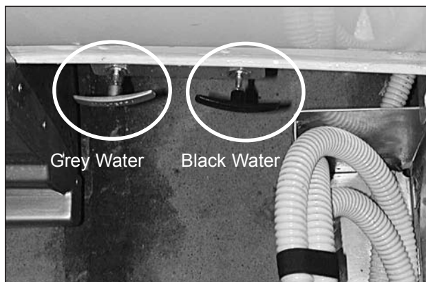
Picture B-P35: Black water, grey water valves and sewage hose locations.
