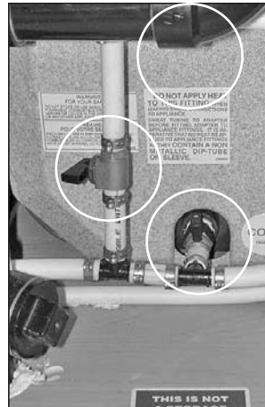
Picture G-P3: Bypass valves mounted at tank in Versatile units (shown in “usage mode”).
