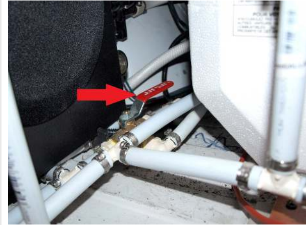
Tank selector lever in the exterior position
