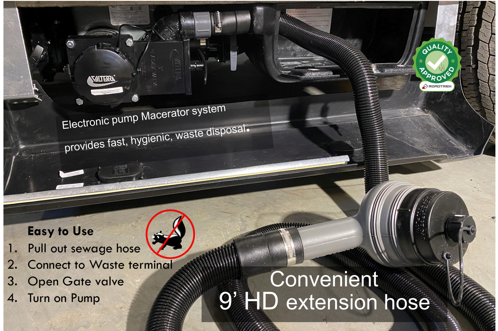
Touch a button to activate Macerator pump
