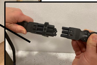
Weiland Connectors allow for cabinet module wiring to be completed in the cabinet shop. Final electrical can be easily connected to the primary electrical harness once the cabinet module is installed in the Roadtrek.
